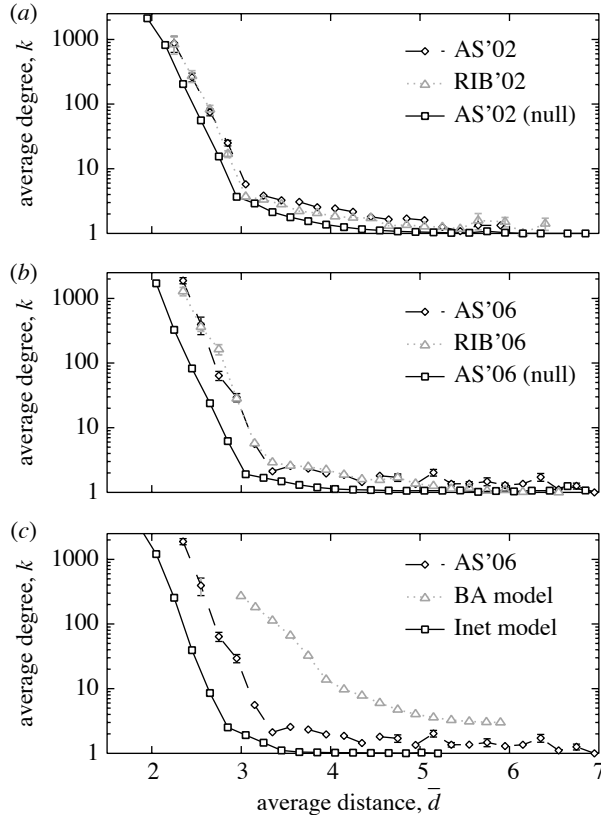
Figure 2. Degree k as a function of the average distance \bar{d} . The panels and symbols are the same as given in figure legend 1.
