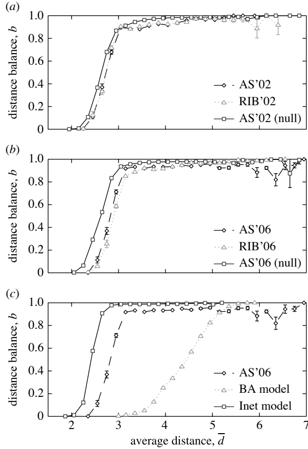
Figure 6. Distance balance b as a function of the average distance \bar{d} . The panels and symbols are the same as given in figure legend 1.
