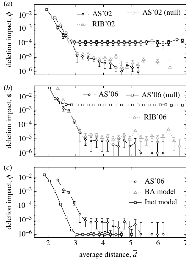
Figure 4. Deletion impact \phi as a function of the average distance \bar{d} . The panels and symbols are the same as given in figure legend 1.
