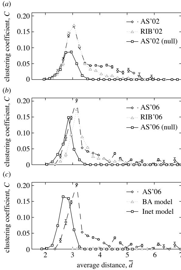
Figure 5. Clustering coefficient C as a function of the average distance \bar{d} . The panels and symbols are the same as given in figure legend 1.
