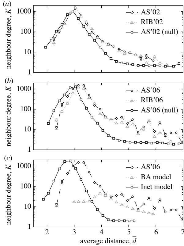
Figure 3. Neighbour degree K as a function of the average distance \bar{d} . The panels and symbols are the same as given in figure legend 1.
