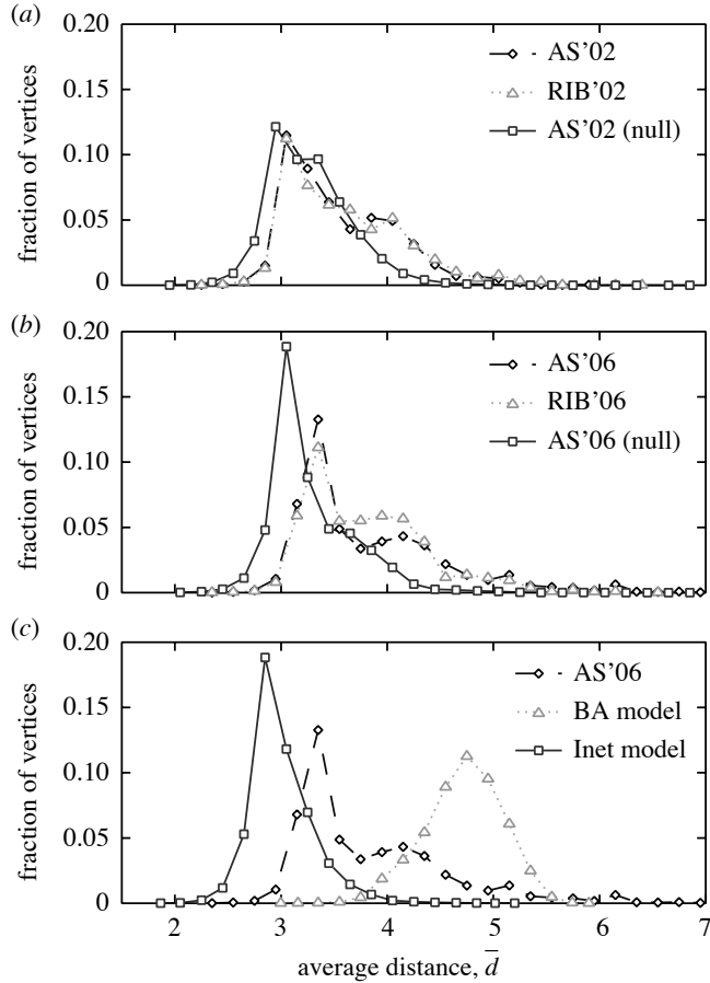
Figure 1. Normalized histograms of vertices with a specific average distance \bar{d} to the rest of the vertices. (a) shows curves for the Oregon Route Views data (RIB'02), extended data (AS'02) and values for random networks with the same degree sequences as AS'02. (b) displays curves for the Oregon Route Views data (RIB'06), extended data (AS'06) as well as randomized networks with the degree sequence of AS'06. (c) shows the same AS'06 curve as (b) along with the BA and Inet model results for parameter values as close as possible to those of the AS'06 network. For the null-model curves in (a) and (b) as well as the model networks in (c), 100 averages were used. Lines are guides for the eyes. The error bars represent standard error (the point symbols are often larger than the error bars).
