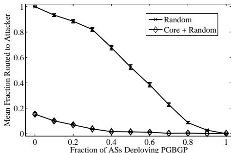
Fig. 3. Both Deployments, Sub-Prefix Hijack, Day One
