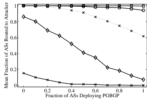
Fig. 6. Core + Random Deployment, Sub-Prefix Hijack, 5 Days
