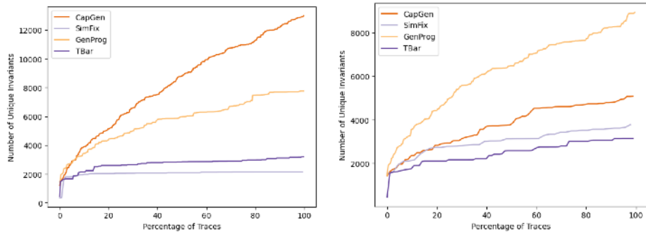
(a) Each tool’s unique invariant accumulation for the first 600 mutants (b) Each tool’s unique invariant accumulation for 1000 randomly sampled mutants
