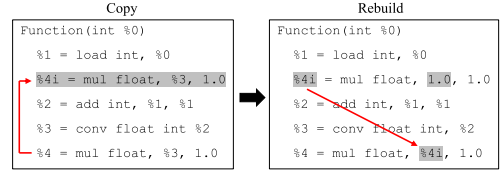
Fig. 4. Mutate-Copy: Operand dependency is rebuilt to preserve LLVM-IR program validity. Since LLVM-IR is strongly typed, the constant value 1.0 is used if no other value in the requested type is available.
