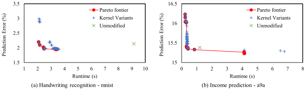
Fig. 11. Pareto-frontiers and other kernel variant measurements for (a) the handwriting recognition (SVM with MNIST) and (b) the income prediction (SVM with a9a).
