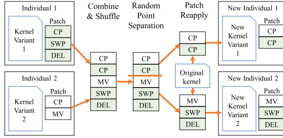
Fig. 5. One-point messy crossover.
