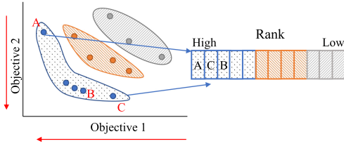
Fig. 3. Non-dominated sorting.
