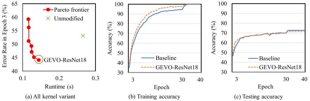
Fig. 13. (a) Pareto-frontiers for the image classification (ResNet18 with CIFAR-10). The kernel in the circle is manually selected to retrain the model until model converges with its (b) training accuracy and (c) testing accuracy across epochs.
