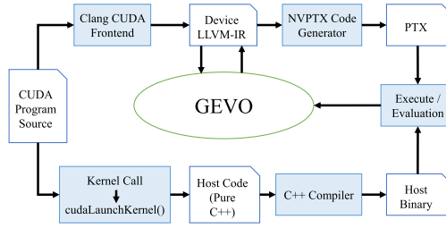
Fig. 2. GEVO in the LLVM/Clang compilation flow.
